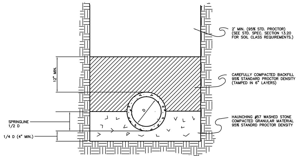
CLASS B COMPACTED GRANULAR BEDDING LOAD FACTOR 1.9
